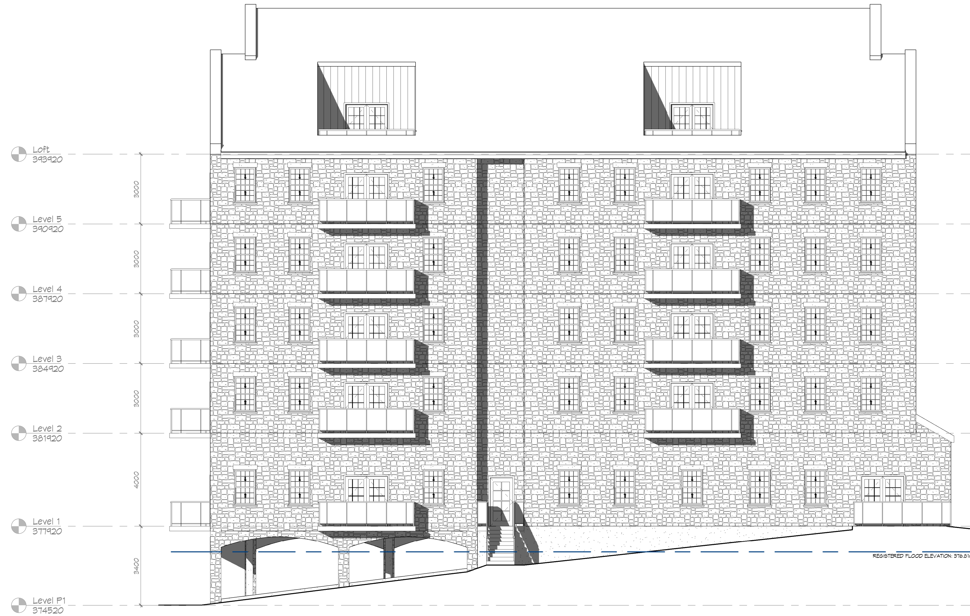
1 Building Elevation East A4.1 1 : 100
